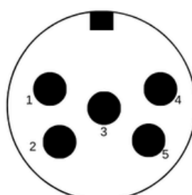
5 pins
